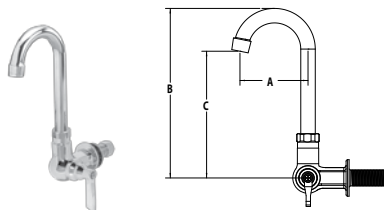
TLL70 Series Single Hole Wall Mount Faucet with Gooseneck Spout
