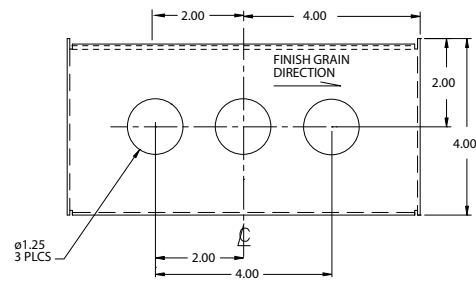
4" OC DECK MOUNT-3 Hole Part No. K17-X301-4D4 Complete with bracket Quantity: _____
