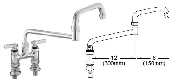
4" (102mm) Center with 18" (457mm) Dbl Jointed Swivel Tubular Spout and Lever Handles
