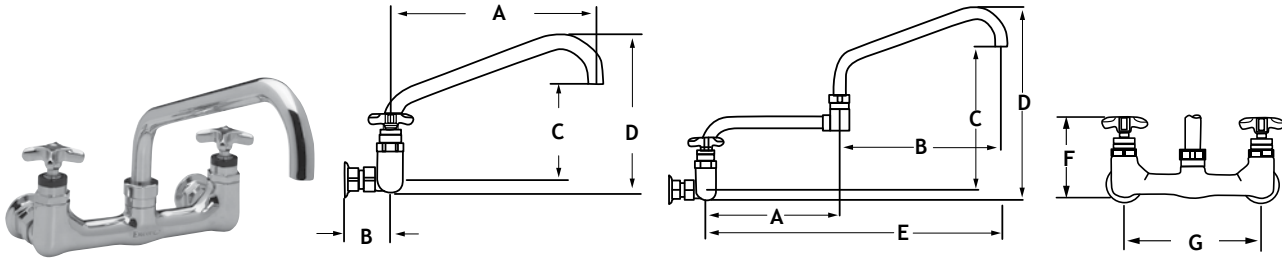
Pot Sink Wall Mount Faucet
