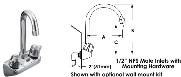
4" (102mm) Wall Mount with Gooseneck Spout and Knob Handles
