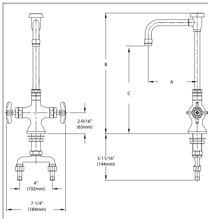
Double Pantry w/8" (203mm) Vacuum Breaker Spout and 4" (102mm) Wrist Blade Handles
