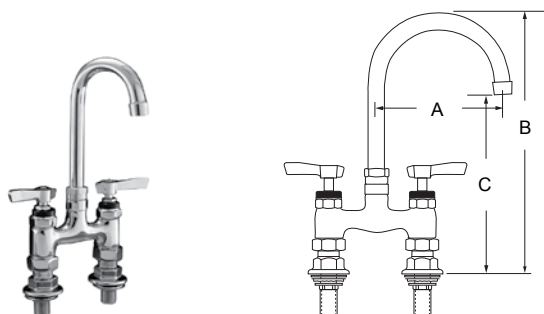
4" (102mm) Center with 3-1/2" (89mm) Gooseneck Spout & Lever Handles
