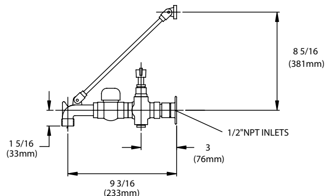
Rough Chrome Service Sink Faucet w/Bracket, Stops, Threaded Spout w/Hook and Lever Handles
