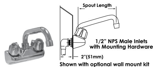
4" (102mm) Wall Mount with Swing Spout and Knob Handles
