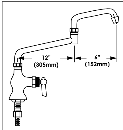
Single Pantry with Double Jointed Spout and Lever Handle
