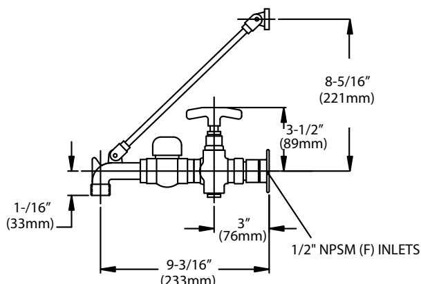
Rough Chrome Service Sink Faucet w/Bracket, Stops, Threaded Spout w/Hook and Cross Handles
