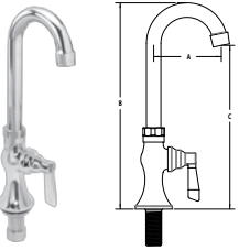
TLL20 Series Single Deck Mount Faucet with Gooseneck Spout
