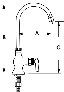
Single Pantry with 8-1/2" (216mm) Swivel and Rigid Gooseneck Spout and Lever Handle
