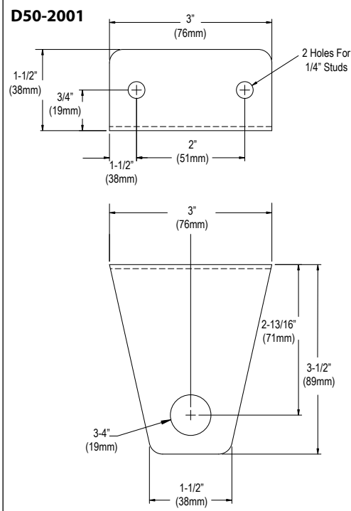
Universal S/S Drain Handle Support For Twist and Rotary Drain Outlets
