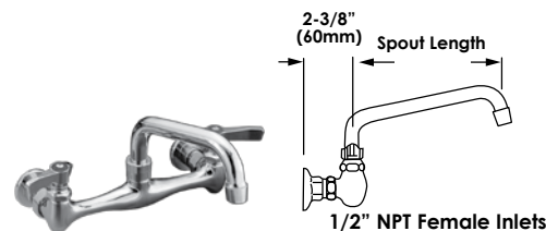
8" (203mm) Wall Mount with Swing Spout and Lever Handles
