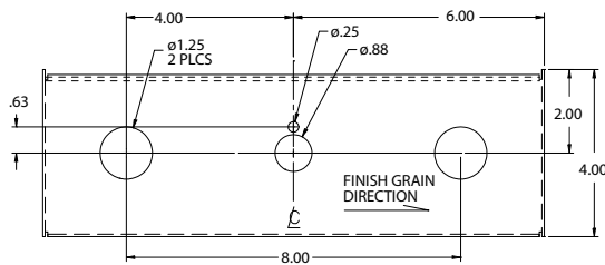
8" OC WALL MOUNT-3 Hole (FOR KL84 SERIES FAUCETS) Part No. K17-X301-8 Complete with bracket Quantity: _____
