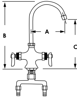
Double Pantry with 8" (203mm) Swivel and Rigid Gooseneck Spout and Lever Handles
