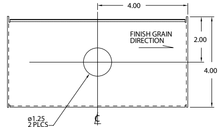
SINGLE HOLE DECK MOUNT Part No. K17-X301-1D Complete with bracket Quantity: _____
