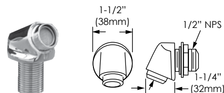
Trough Inlet Fitting
