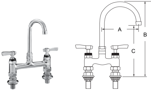
6" (152mm) Center with 3-1/2" (89mm) Gooseneck Spout & Lever Handles
