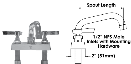
4" (102mm) Deck Mount with Swing Spout and Lever Handles
