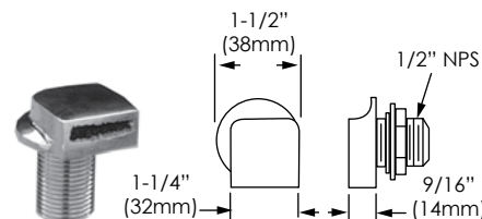
Swirl Inlet Fitting
