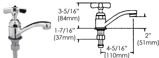
Single Spout Swing Faucet 360° Rotation
