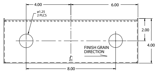
8" OC DECK MOUNT Part No. K17-X301-8D2 Complete with bracket Quantity: _____
