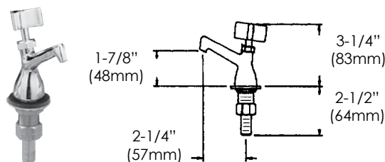
Dipperwell Faucet
