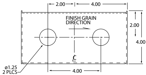
4" OC DECK MOUNT Part No. K17-X301-4 Complete with bracket Quantity: _____
