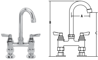
TLL57 Series 4" (102mm) Deck Mount Faucet with Gooseneck Spout
