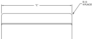
WALL CLIP Part No. K17-X107-1 "L"=7.50" K17-X107-2 "L"=11.50" Quantity: _____ Quantity: _____
