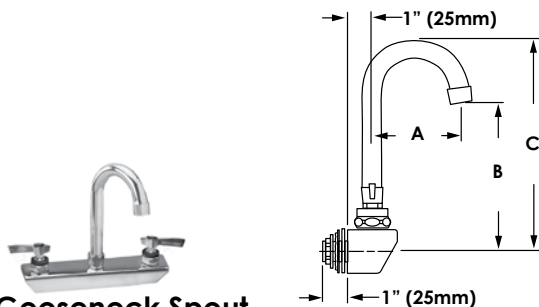
8" (203mm) Wall Mount with 3" (76mm) Gooseneck Spout and Lever Handles
