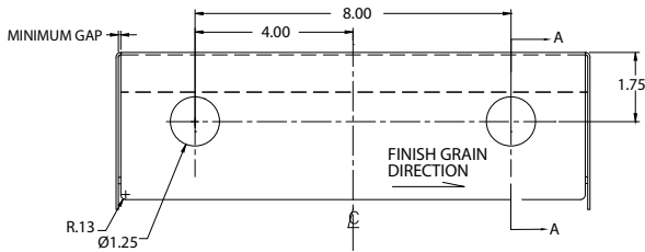
8" OC WALL MOUNT (FOR KL84 SERIES FAUCETS) Part No. K17-X301-8W Complete with bracket Quantity: _____
