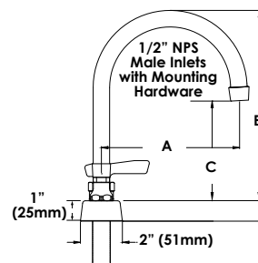
4" (102mm) Deck Mount with Swivel Gooseneck Spout and Lever Handles
