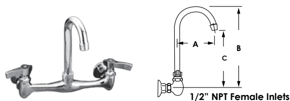
8" (203mm) Wall Mount with Gooseneck Spout and Lever Handle
