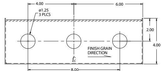
8" OC DECK MOUNT-3 Hole Part No. K17-X301-8D3 Complete with bracket Quantity: _____
