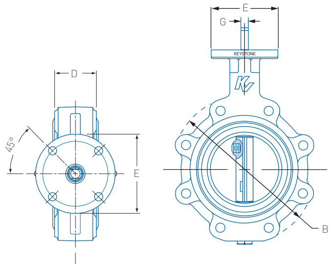
F222 LUGGED STYLE VALVE
