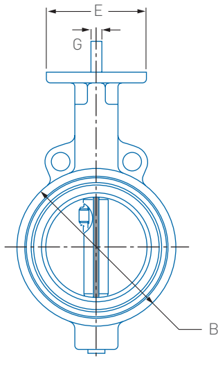
F221 WAFER VALVE
