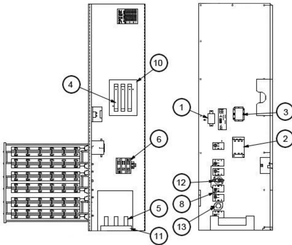
RXJJ-CE20D Assembly
