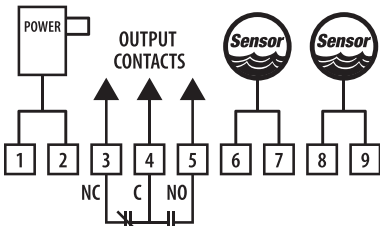
FIGURE 1 – WIRING DIAGRAM
