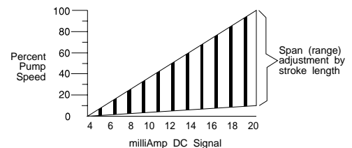
MP-100 Adjustment Range
