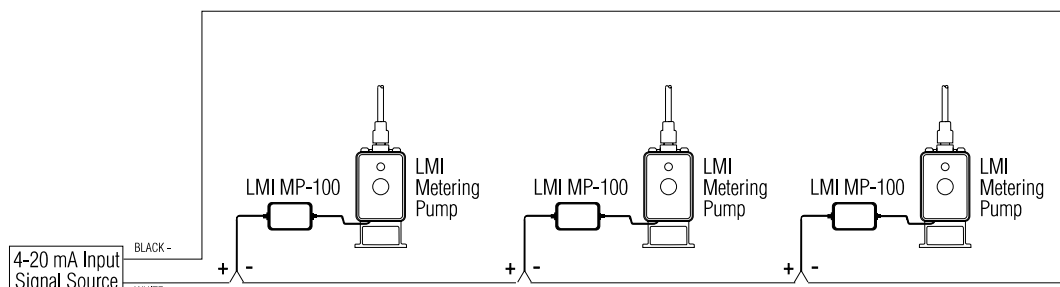
MP-100 Series Loop Control
