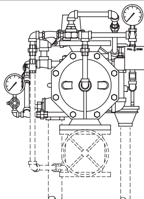
Electric Actuation Shown
