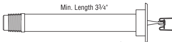
63-121-X-XXX Recessed Horizontal Sidewall w/Std. Escutcheon (1" NPT)
