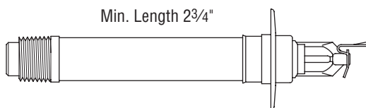
60-95X-X-XXX Extended Coverage Sidewall SR, w/Std. Escutcheon (1" NPT)
