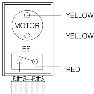
INTERNAL VIEW
