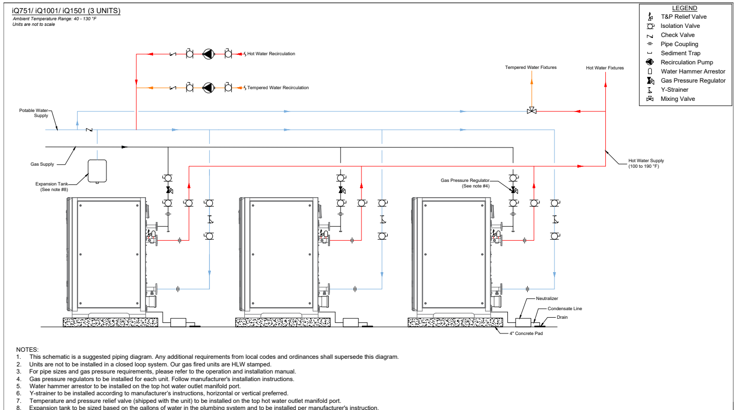
Multiple unit system with mixing valve but no storage tank.
