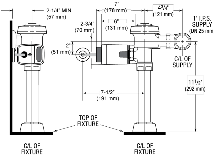
EL-700-A Single-Flush SideMount Hardwired unit shown on an existing Royal 111 closet flushometer
