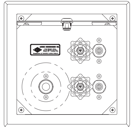
CATALOG #8155 HOT & COLD LESS VACUUM BREAKER w/DOOR
