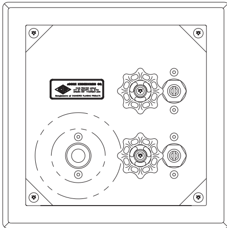
CATALOG #8145 HOT & COLD LESS VACUUM BREAKER
