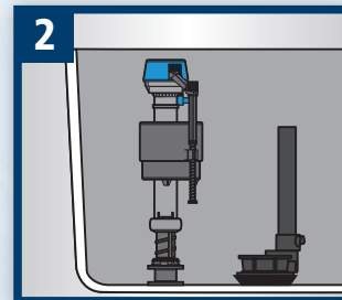
Install Fill Valve
