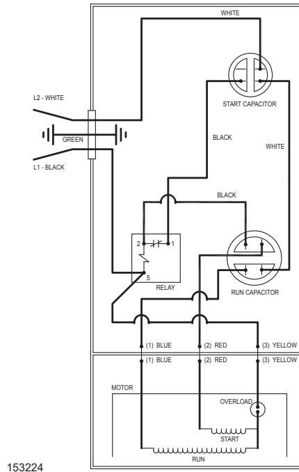
WIRING DIAGRAM FOR MODELS "N803", "N805", "N807", "E803", "E805", "E807" 4/15 thru Current
