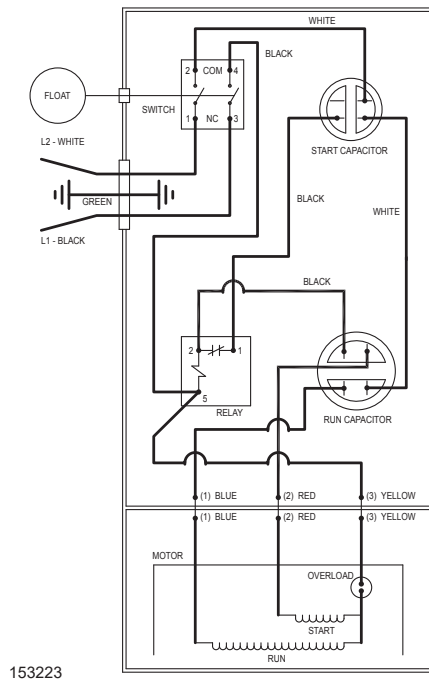
WIRING DIAGRAM FOR MODELS "M803", "M805", "M807", "N803", "N805", "N807", "D803", "D805", "D807" 4/15 thru Current
