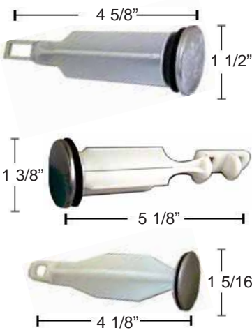
LAVATORY POP-UP STOPPERS
