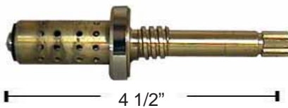
SM401 Fits Temptrol Ea.
