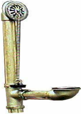
CONNECTED WASTE AND OVERFLOW FOR CLAWFOOT TUB
