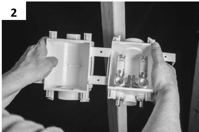
2 Simply slide integrated mounting flanges into opposing box
