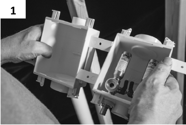
1 To attach multiple boxes, hold boxes at an angle. If installing a single box system skip to step 4a.
