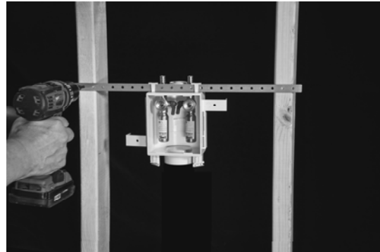
4a Determine box configuration and secure with one of the above methods.
