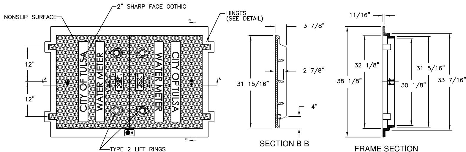
PLAN VIEW
