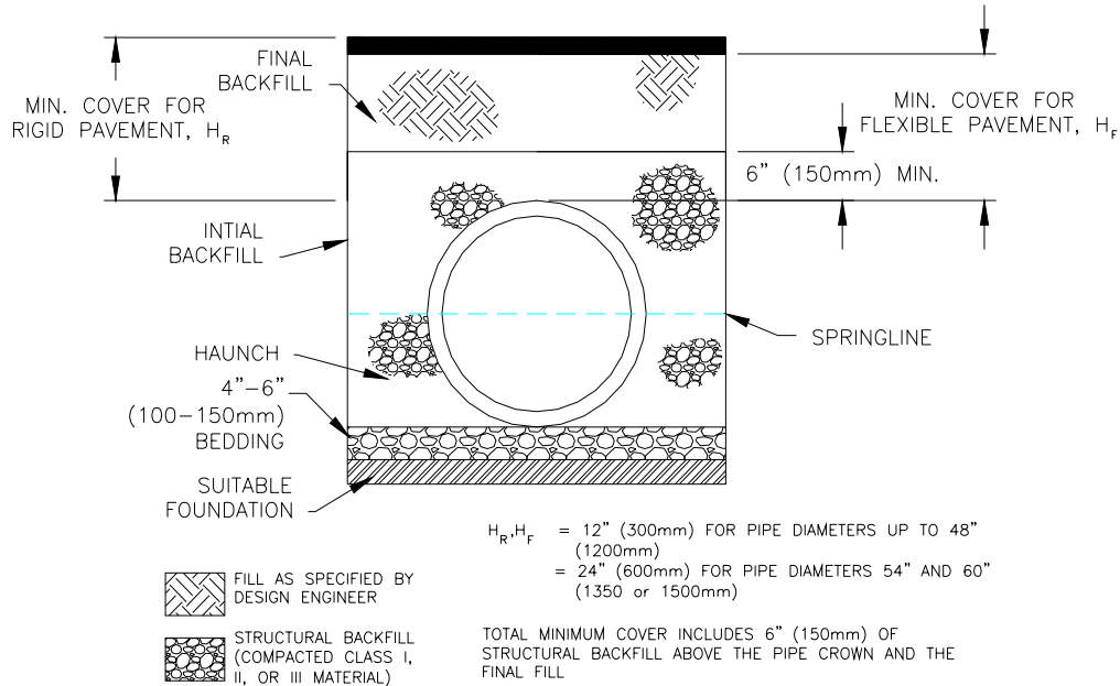
Figure 1 Typical Backfill Structure
