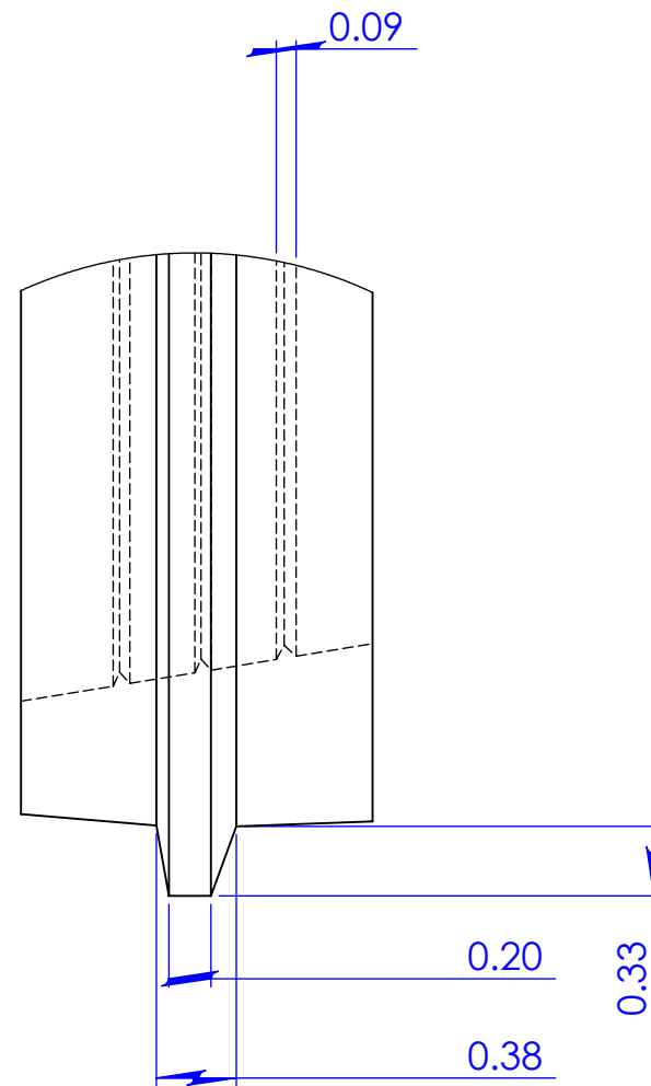
DETAIL C SCALE 1 : 1
