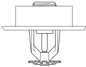
Note: TY-B Standard Response 1/2" NPT K=5.6 Sprinklers is shown
