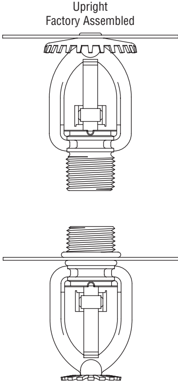
*Pendent Shown Field Assembled (Order 53-112-X-XXX Sprinkler and Shield Assembly Separately)
