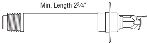
60-35X-X-XXX Extended Coverage Sidewall QR, w/Std. Escutcheon (1" NPT)
