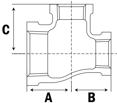
Bronze Reducing Tee - 72230
