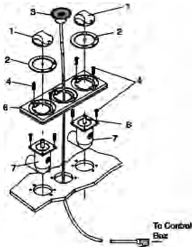
3-Hole Control Panel with Center Bath Control
