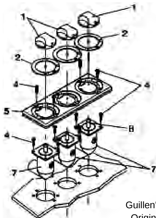
3-Hole Control Panel with 3 Air Controls
