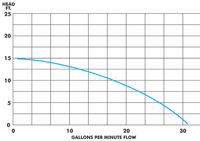
YELLSUB Performance Curve 1 1/4" - 3/4" Discharge
