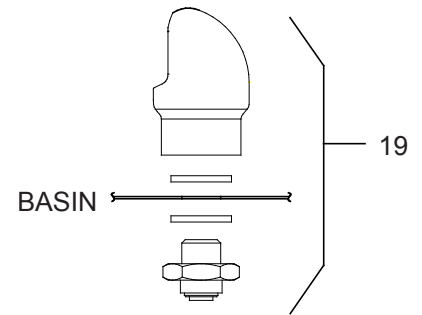
Bubbler Detail
