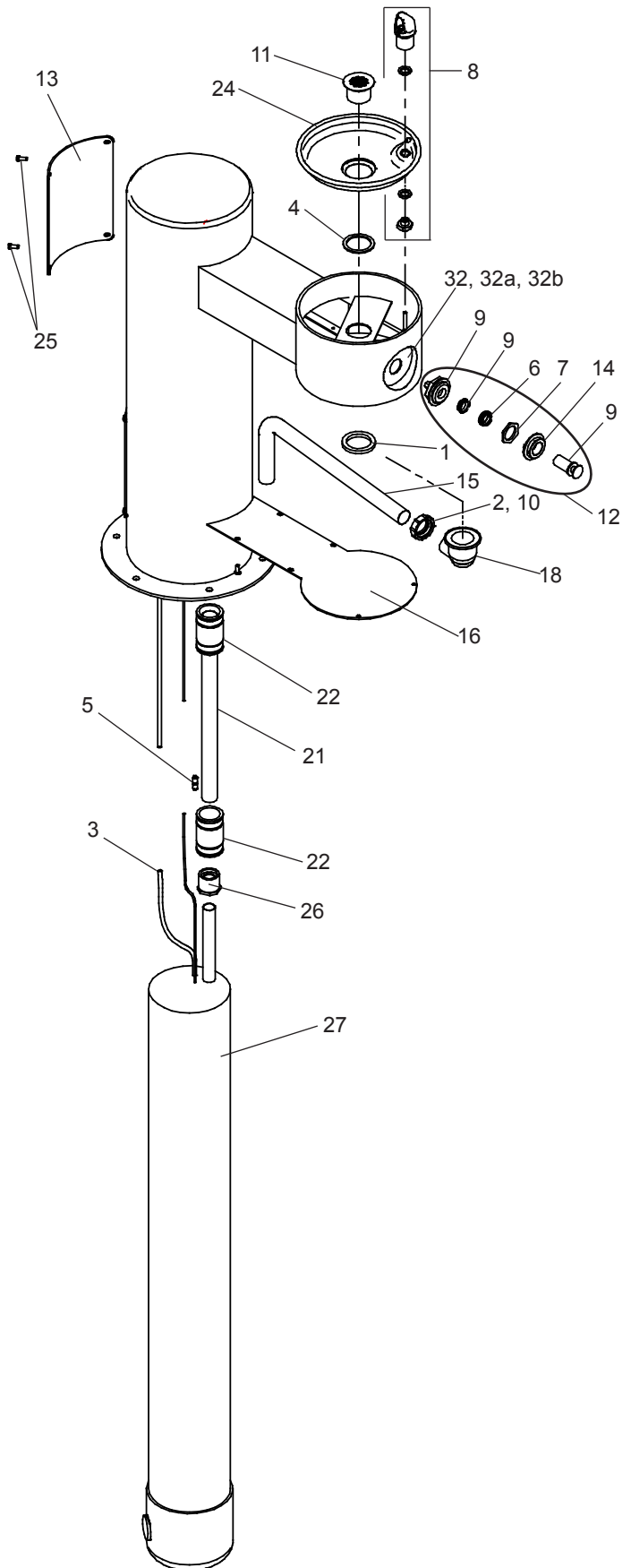
Single Valve Assy. (Item 28)
