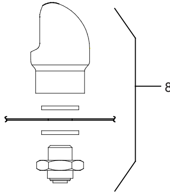
Vandal Resistant Bubbler Detail
