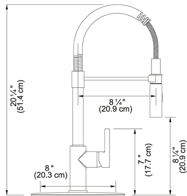
Technical Drawing
