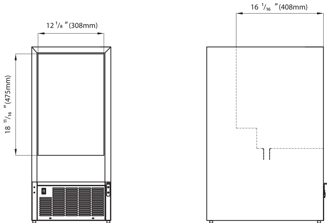
Front View
