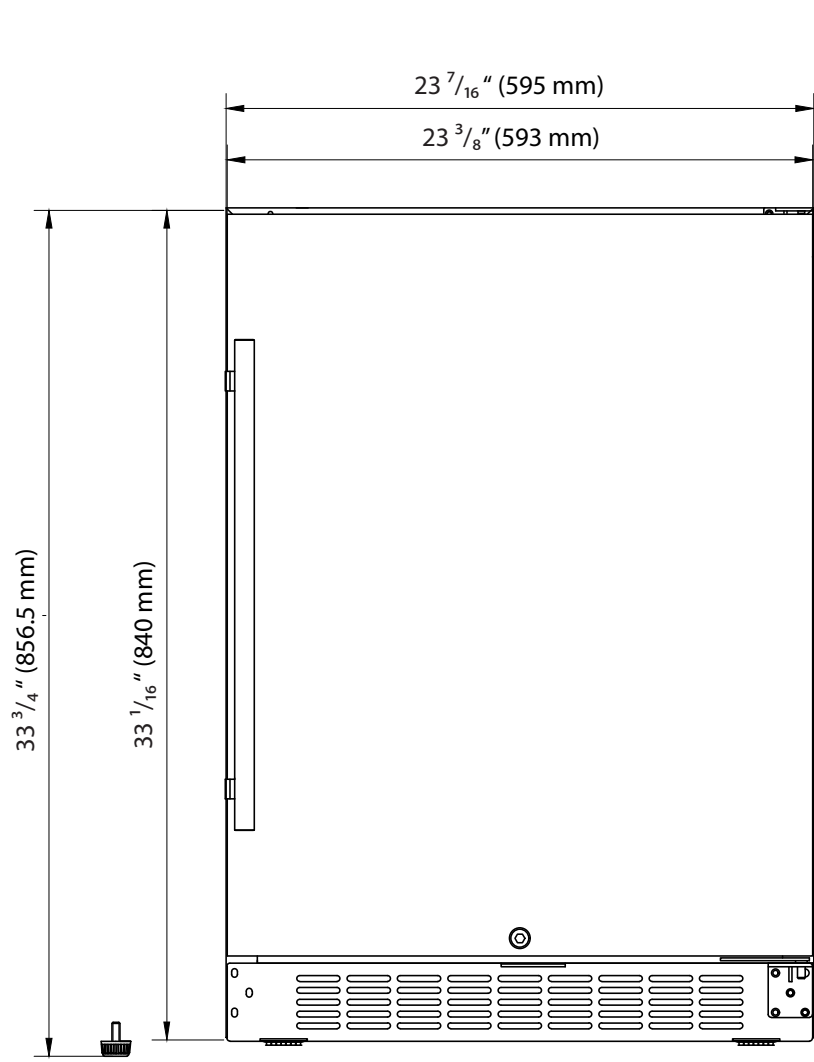
Front View
