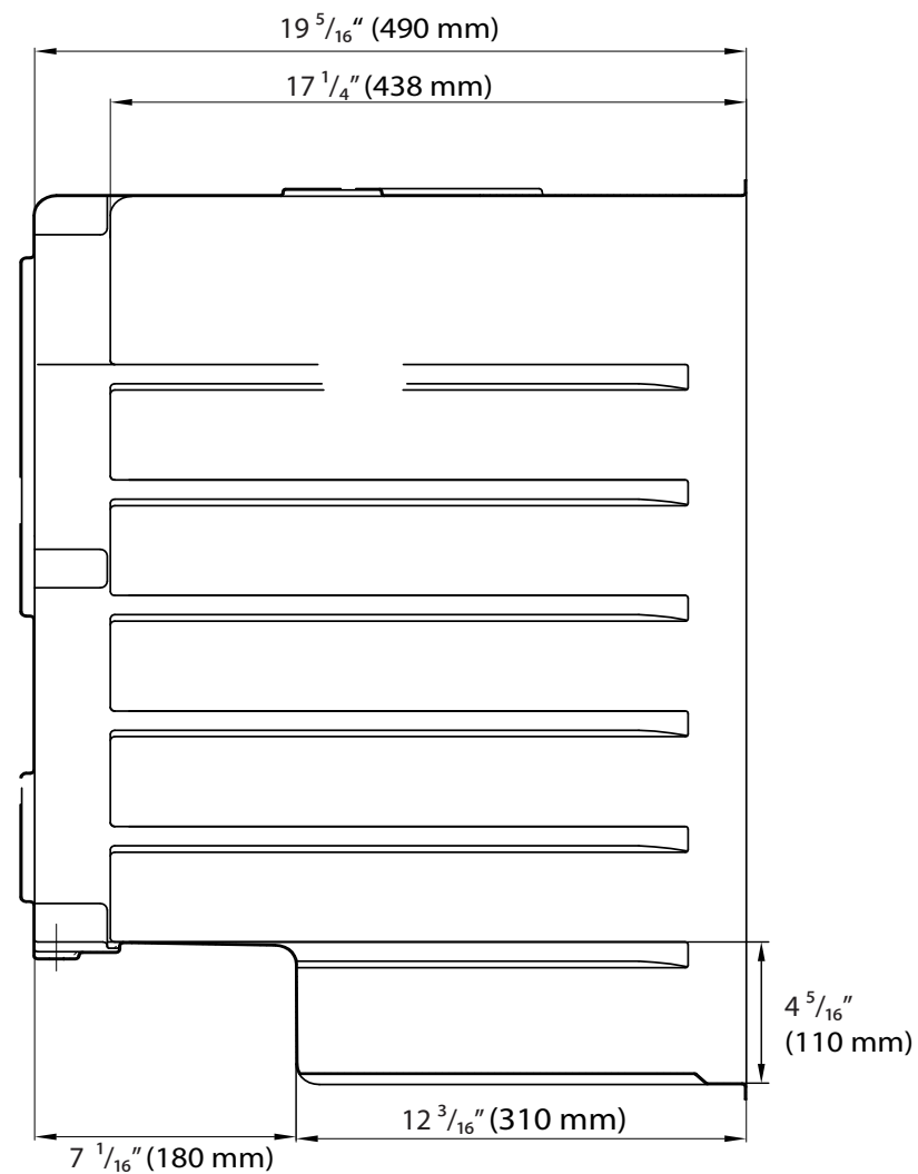
Side View
