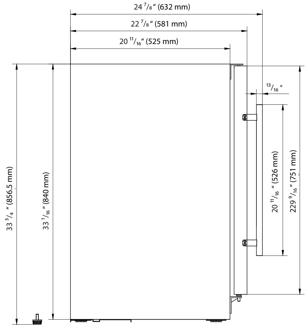
Side View
