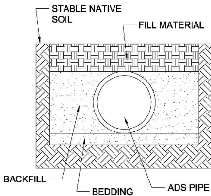
Figure 3: Rectangular Trench Installation
