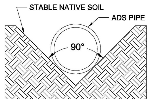
Figure 1: V-Bottom Trench
