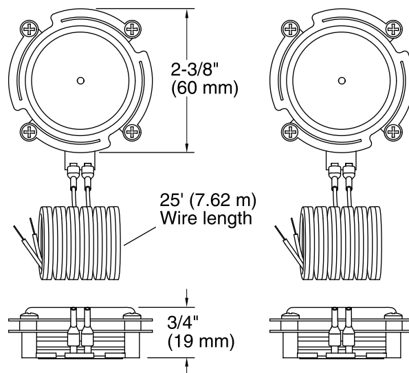
Speakers - Includes 2
