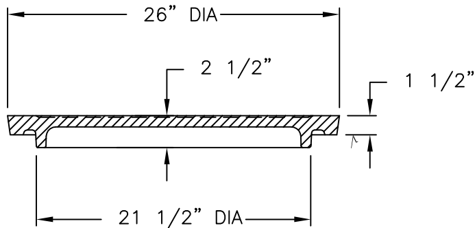
COVER SECTION
