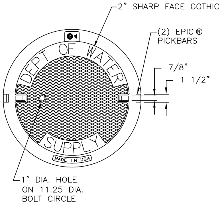
PLAN VIEW
