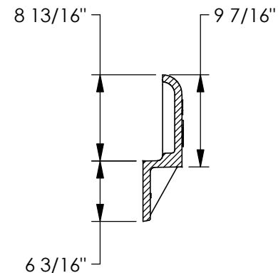
SECTION C-C SCALE 1 : 14
