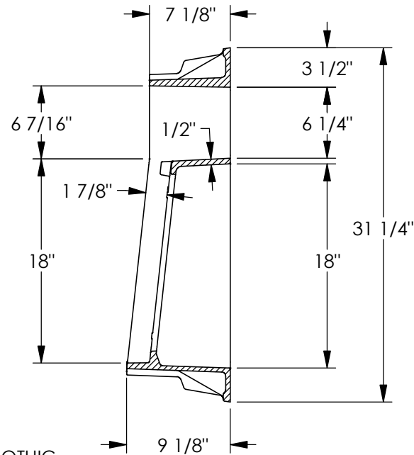
SECTION B-B
