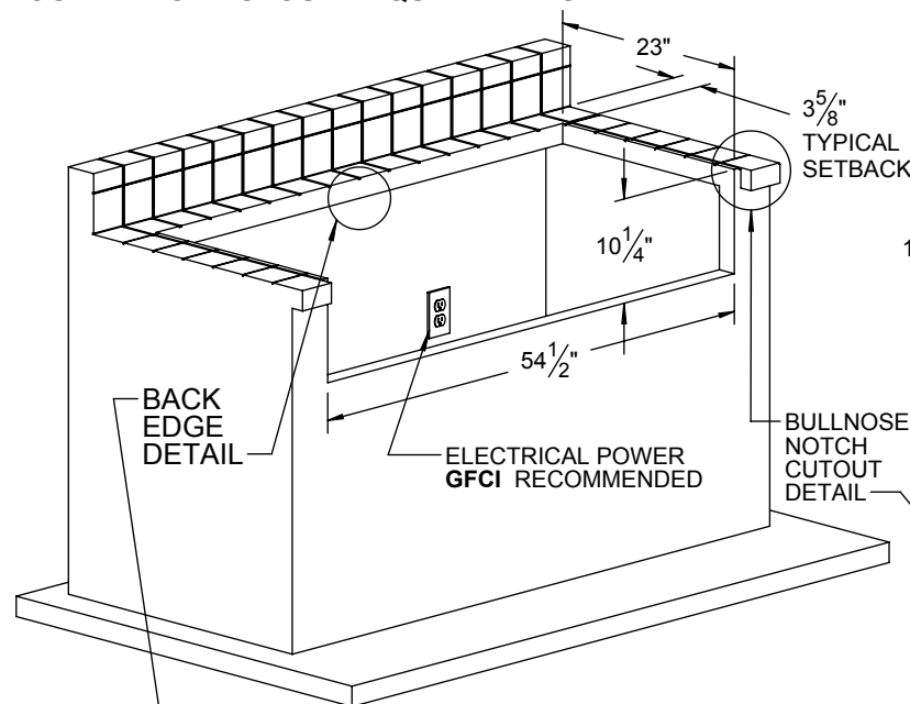
TYPICAL ALX2-56 BFG INSTALLATION
