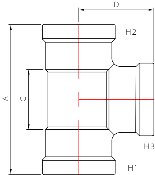
INJECTION MOLDED FITTING (M)
