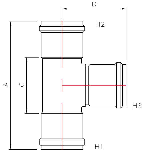
FABRICATED FITTING (F)
