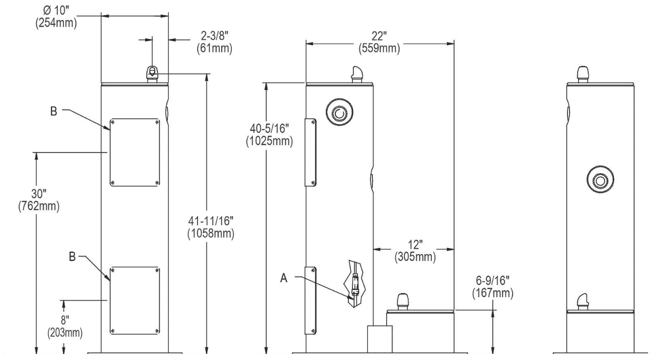
BACK VIEW
