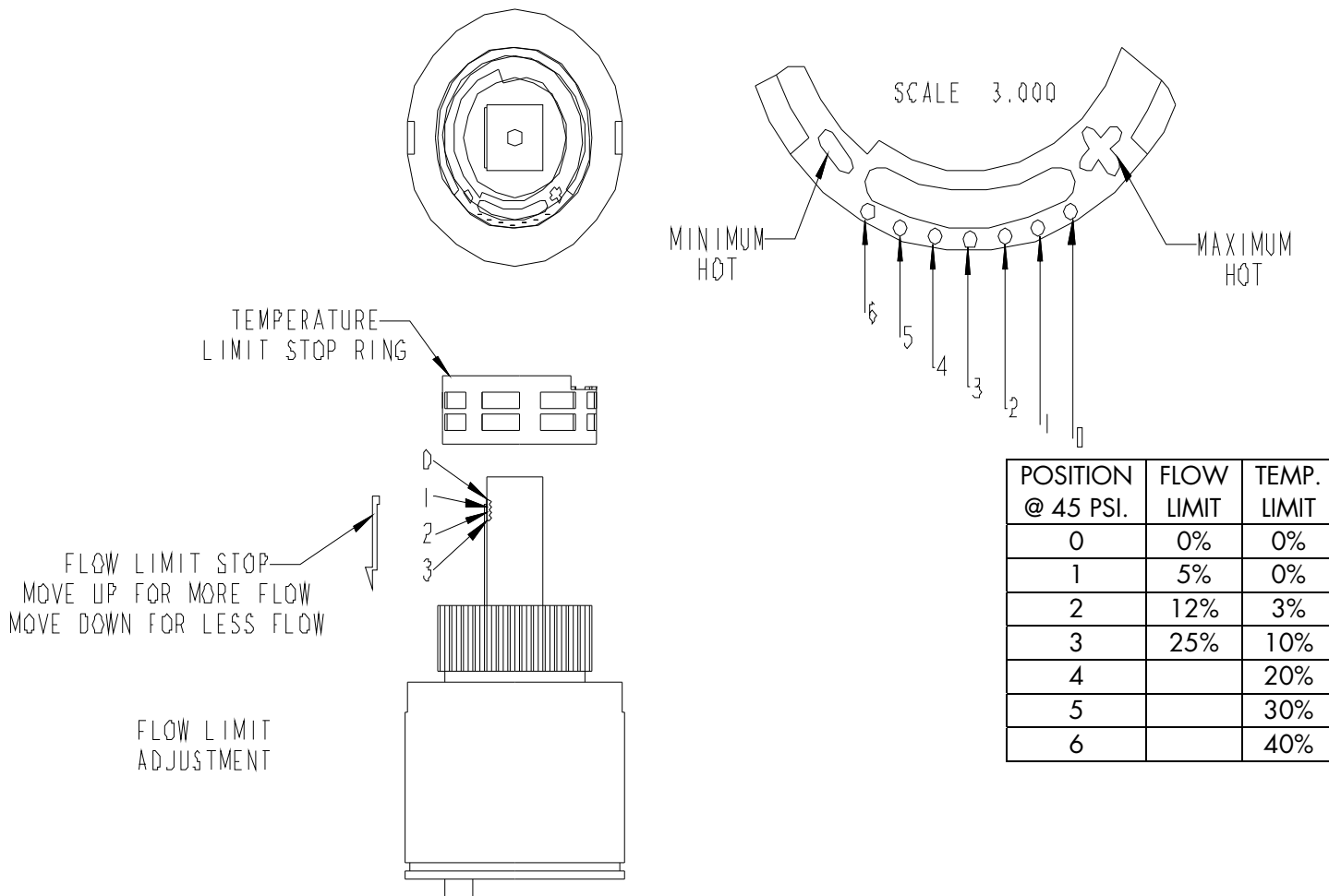
TEMPERATURE LIMIT STOP RING ADJUSTMENT
