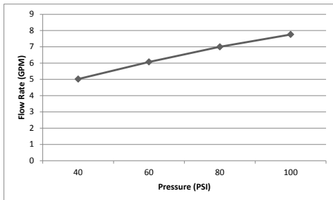
P-2300B Flow Rate (GPM) Vs Pressure (PSI) For Tub Port*
