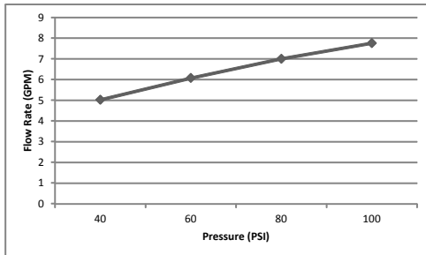
P-2400B Flow Rate (GPM) Vs Pressure (PSI) For Tub Port*
