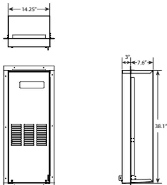
Recess Box for New Construction: 100266730
