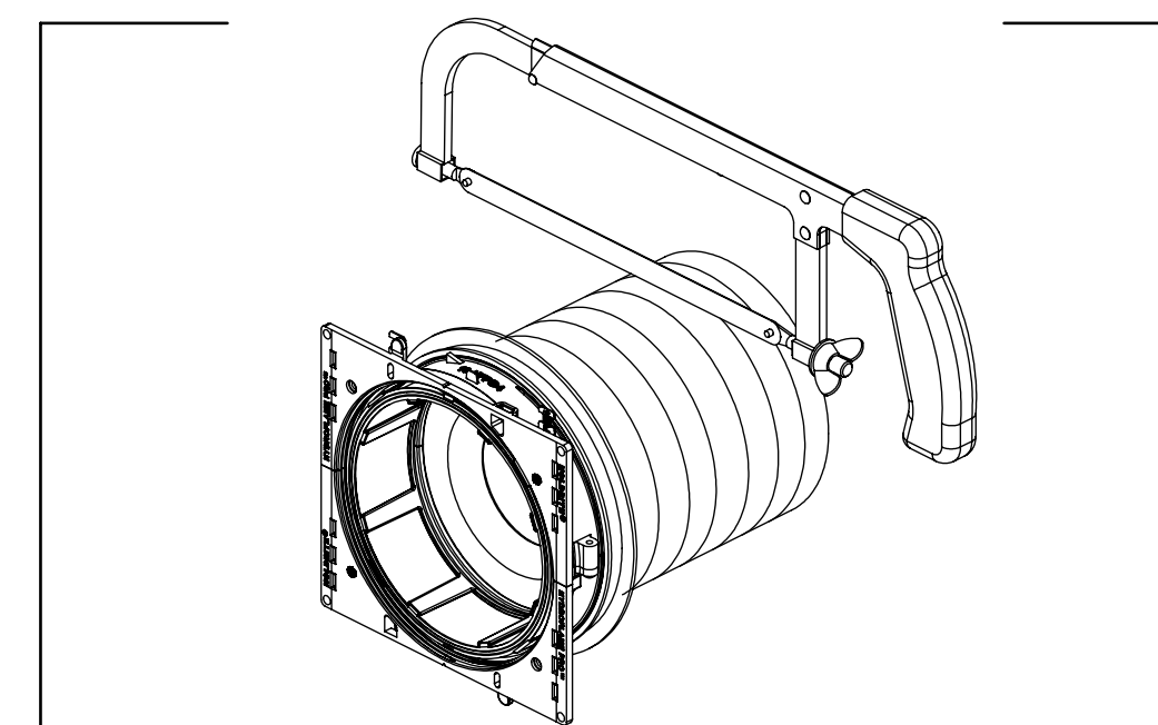
CUT INNER & OUTER SLEEVE AS NEEDED, TO ACCOUNT FOR AERATOR BOX HEIGHT. (CAN BE CUT AS SHORT AS 2-1/2") (Fig. 2)
