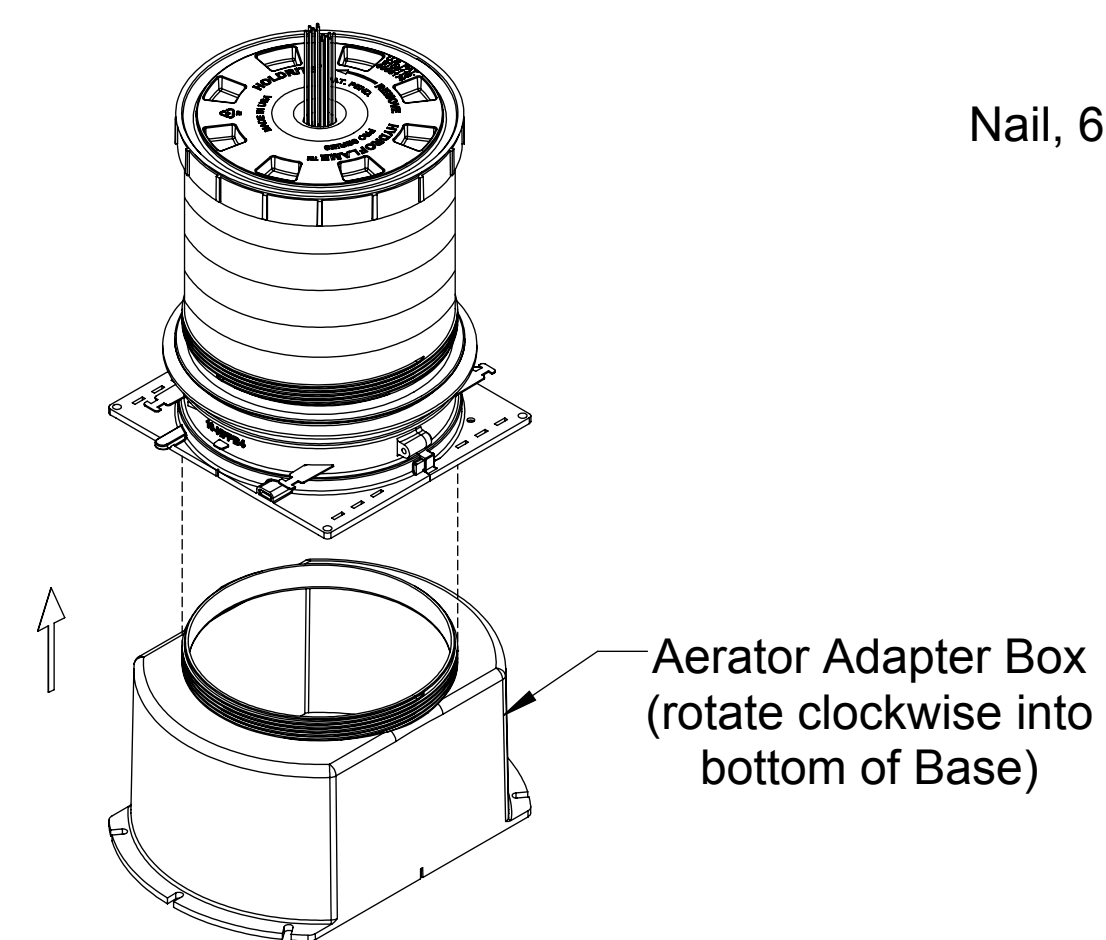
INSTALL AERATOR ADAPTER BOX. (Fig. 5)
