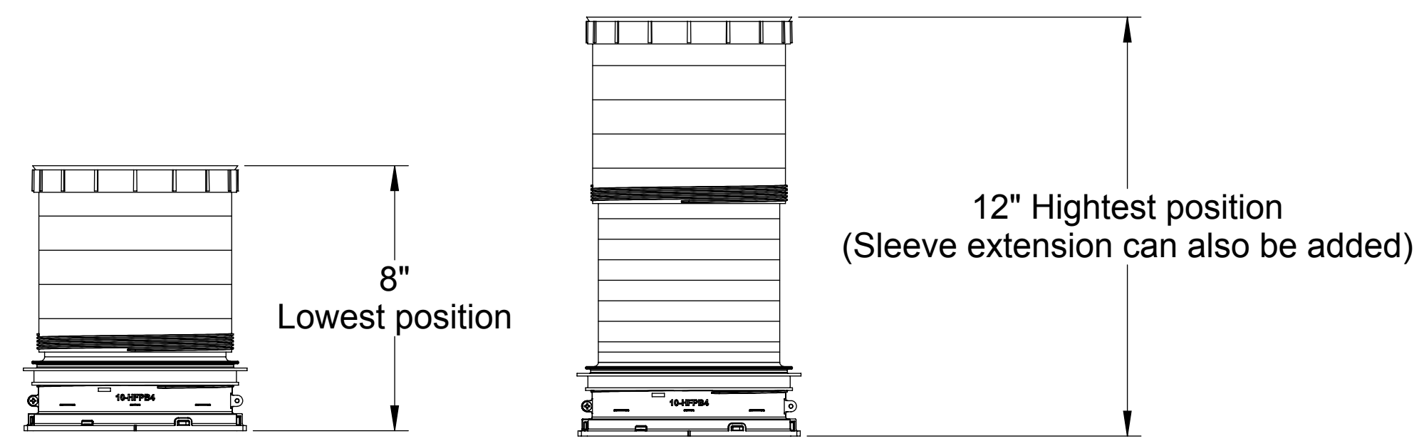
ADJUST TO DESIRED HEIGHT, ACCOUNT FOR AERATOR BOX HEIGHT. (Fig. 1)
