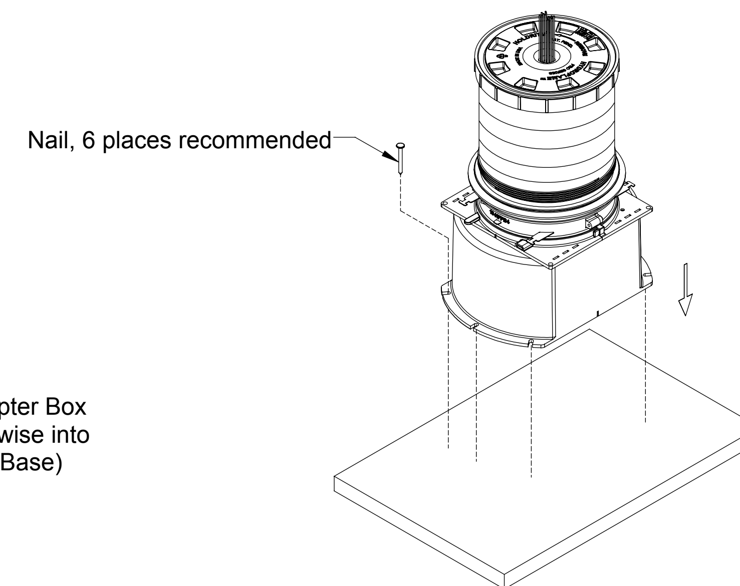
NAIL TO FORM DECK. (Fig. 6)
