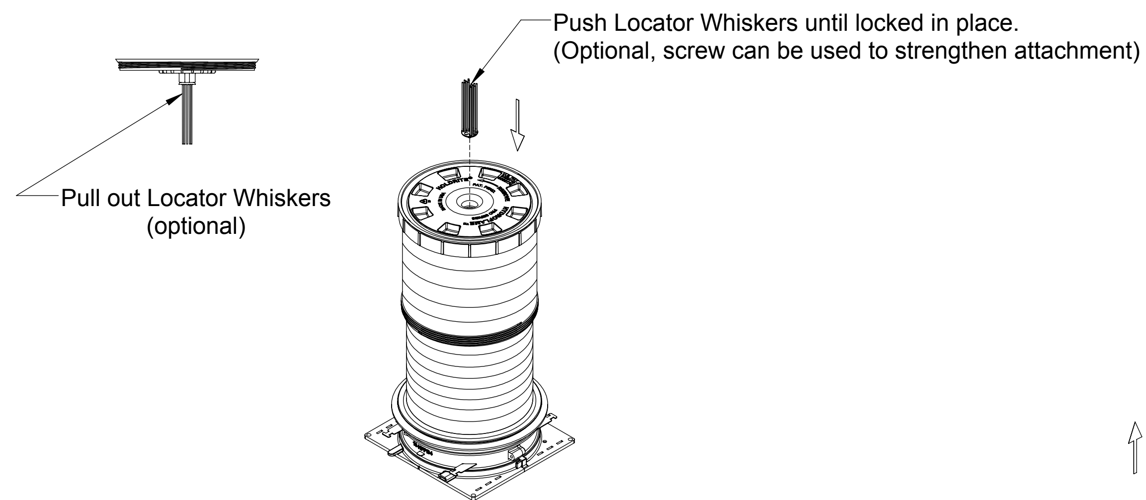
RE-INSTALL CAP & INSERT LOCATOR WHISKERS. (Fig. 4)
