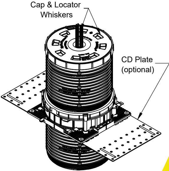
Safety Cap & Locator Whiskers Included (Shown with optional CD Plate) (OSHA Compliant Hole Cover)
