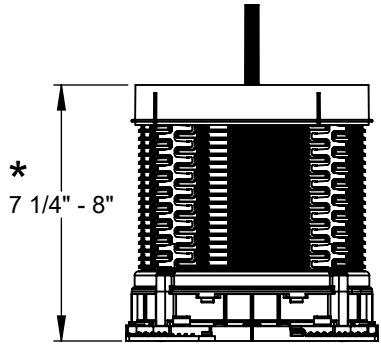
("B") Series Firestop Sleeves (7-1/4" thru 8") with Adjustable Cap
