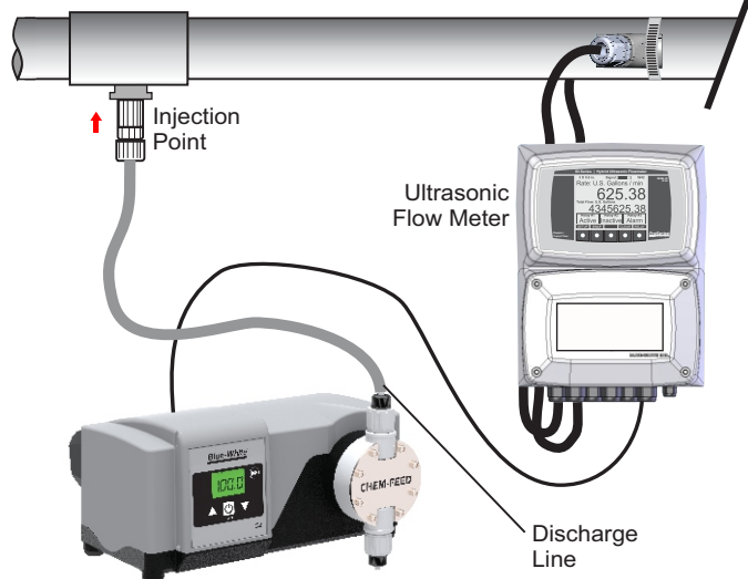
Example #1, Ultrasonic flow meter
