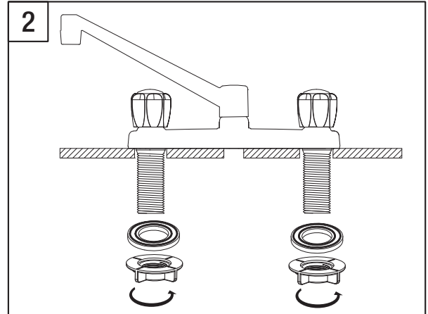
Screw and tighten washer and lock nut onto faucet.
