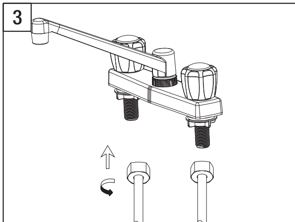
Attach water supply lines (not included) to the faucet.
