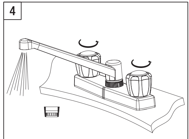
After installing faucet, remove aerator and turn on water to remove any left over debris. Re-assemble aerator.
