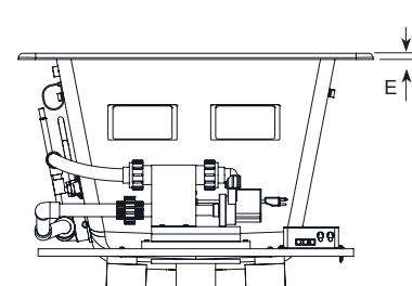
End View
