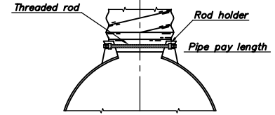
TYPE 2 CONNECTIONS
