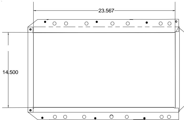
Figure 1 Filter Dimensions
