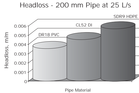
Figure 2 – Pipe Material
