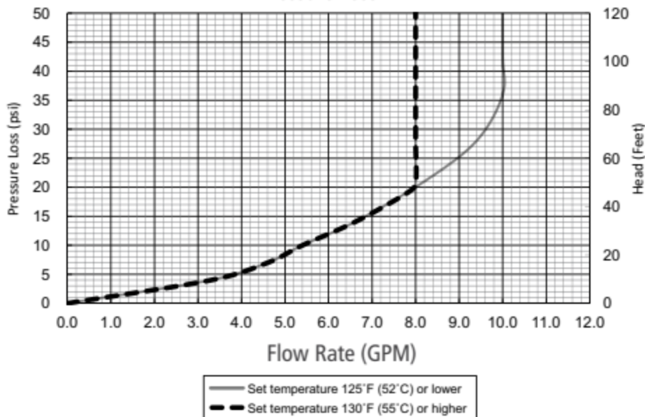
Pressure Loss
