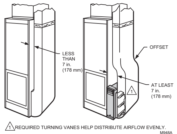
Fig. 13. Typical use of duct offset to provide space for media air cleaner.
