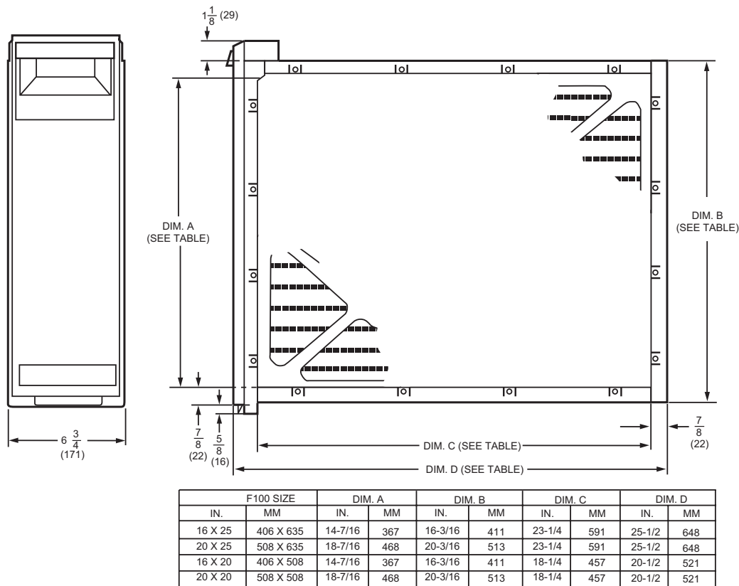
Fig. 1. Installation dimensions in in. (mm) of air cleaner.
