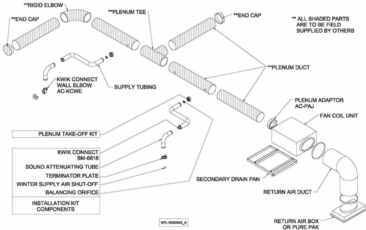
SPACEPAK DESCRIPTION: PLENUM TAKE OFF ROUND SHEET METAL DUCT DWG NO.: SPL-WG0949 REV.: A
