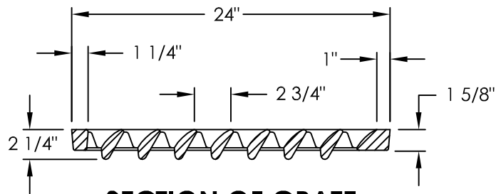
SECTION OF GRATE
