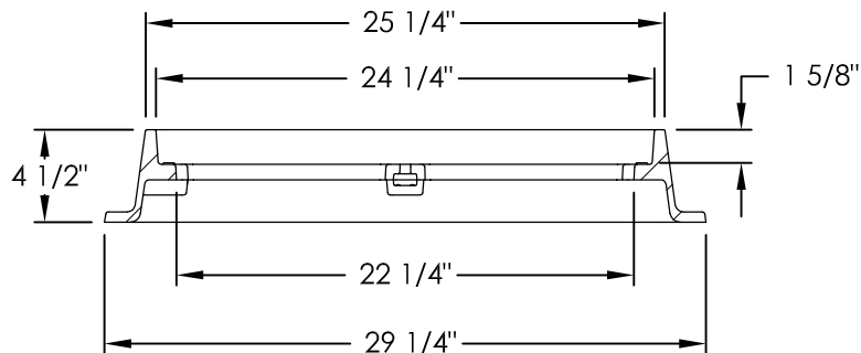
FRAME SECTION VIEW
