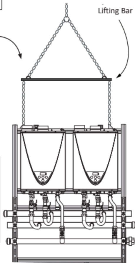
Figure 2: Spreader Lifting Bar
